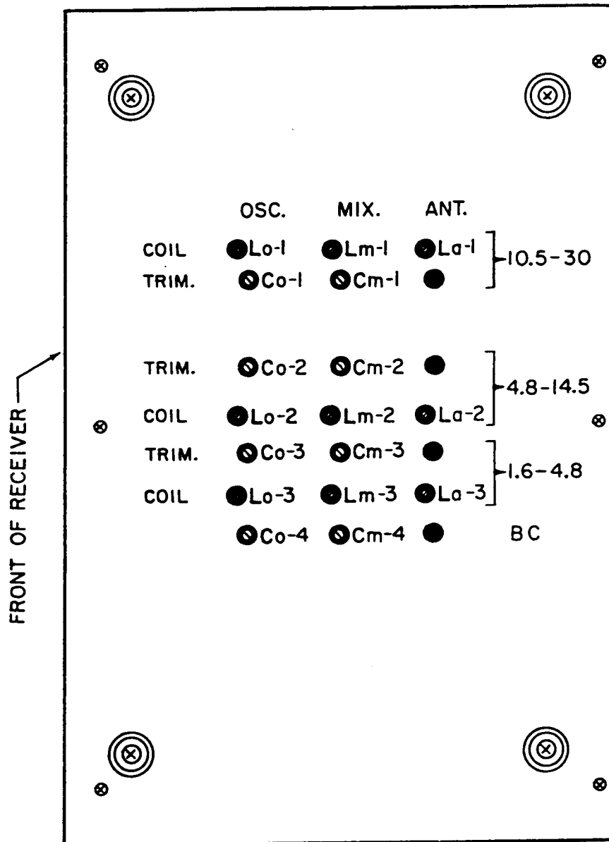
LOCATION OF RF ADJUSTMENTS
