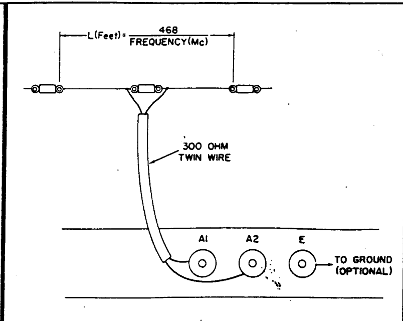
FIGURE 2 Doublet Antenna
