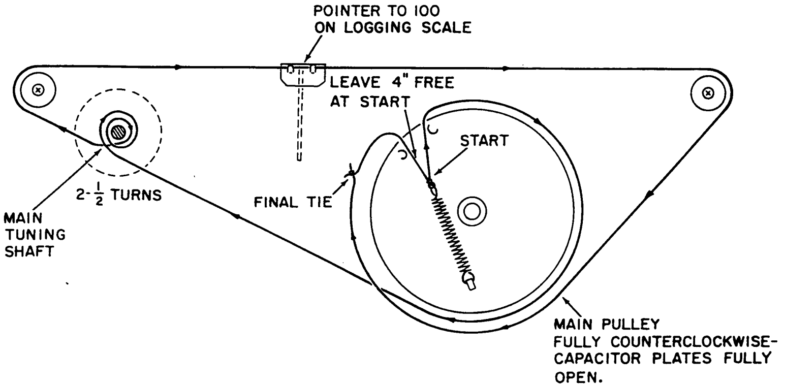
MAIN TUNING DIAL CORD STRINGING
