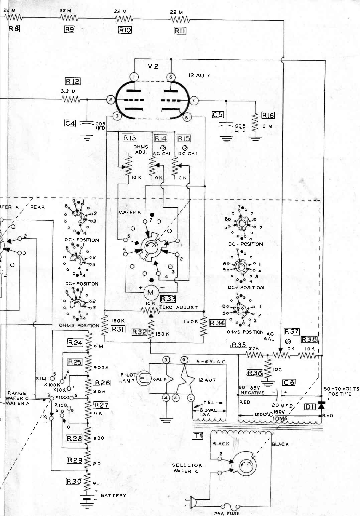
KIT SERVICE BENCH VTVM MODEL IM-10
