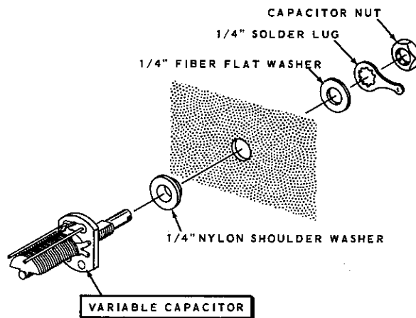
Detail 3-6A
