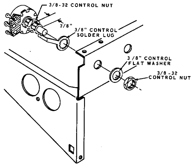
Detail 2-2W
