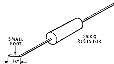
Detail 3-4B
