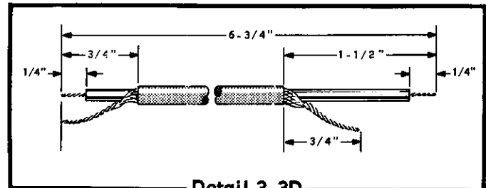
Detail 3-3D
