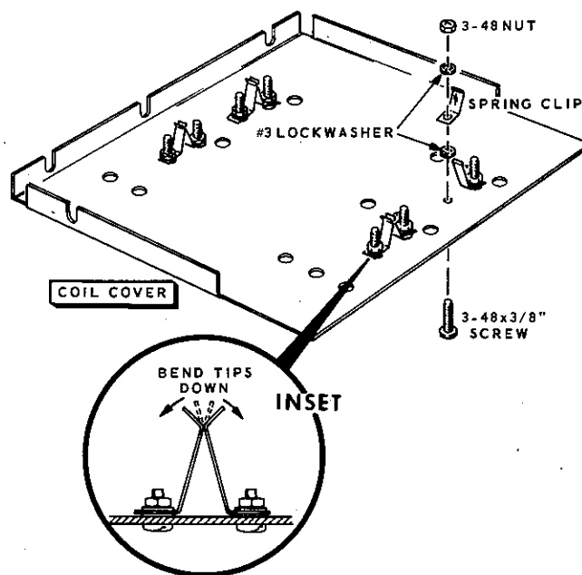
PICTORIAL 3-27
