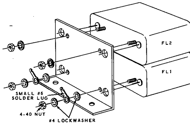
Detail 2-2L
