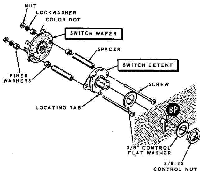
Detail 3-2A
