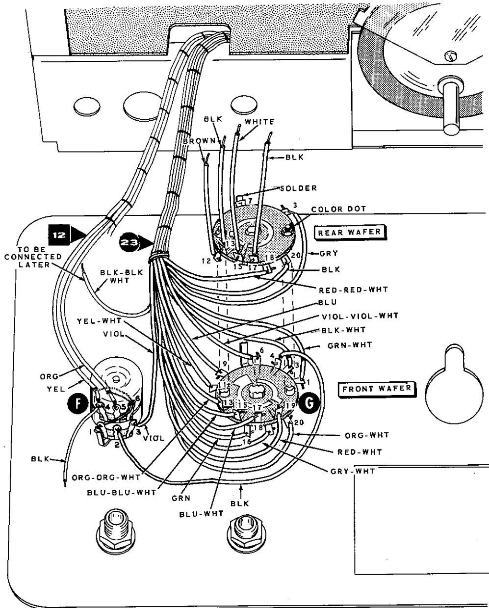
PICTORIAL 3-14
