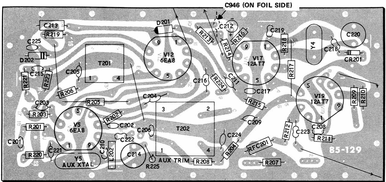
BANDPASS CIRCUIT BOARD #85-129-4
