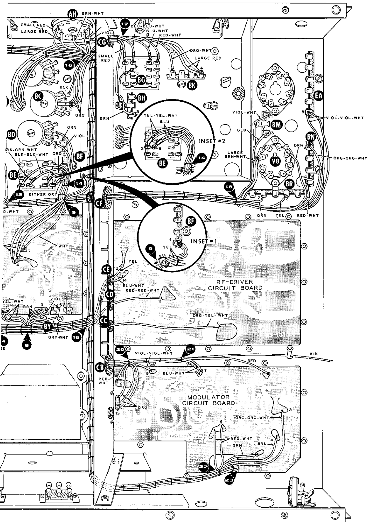
PICTORIAL 3-1
