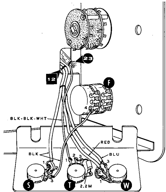
PICTORIAL 3-18
