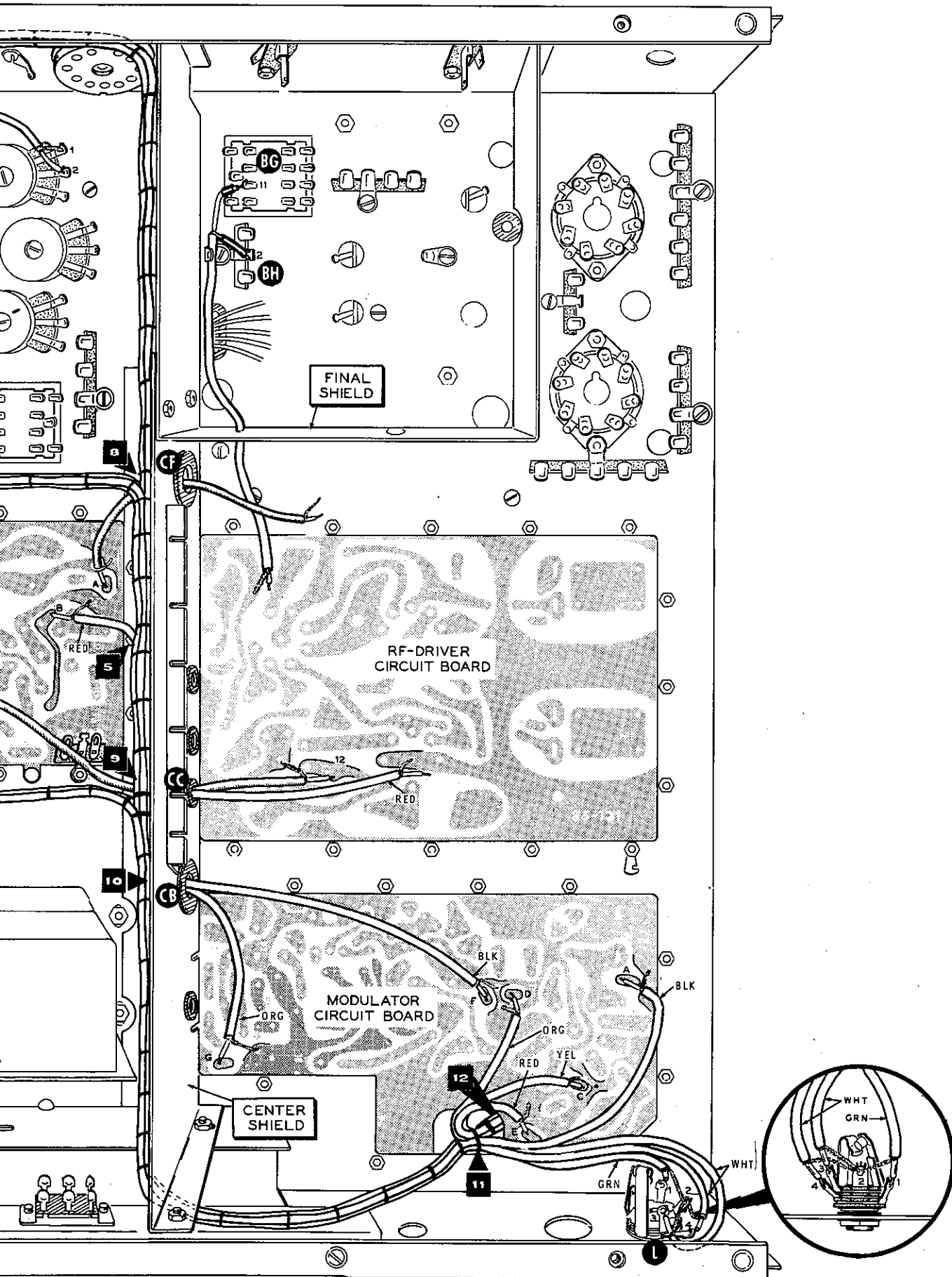
PICTORIAL 3-3
