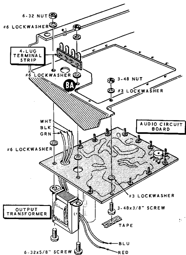
Detail 2-2J
