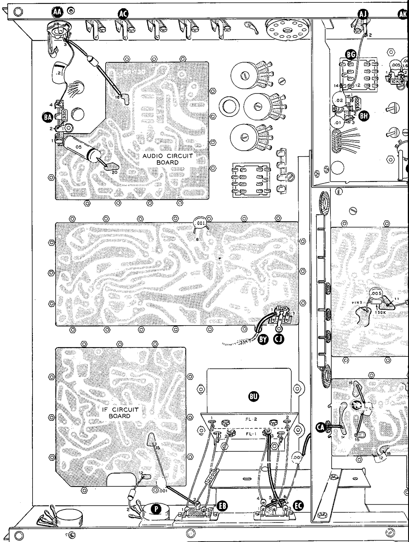
PICTORIAL 3-4
