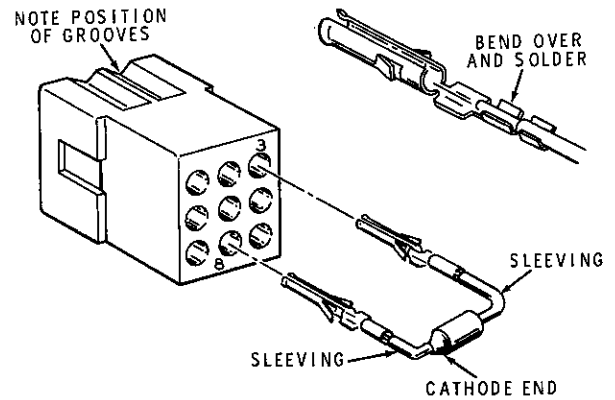
Detail 3-17B
