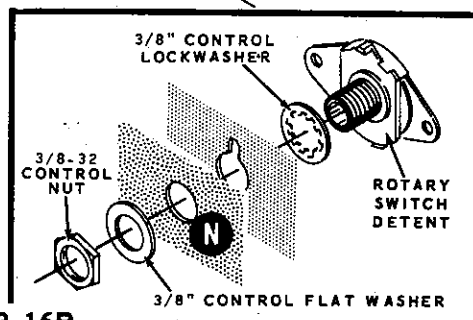
Detail 3-16B
