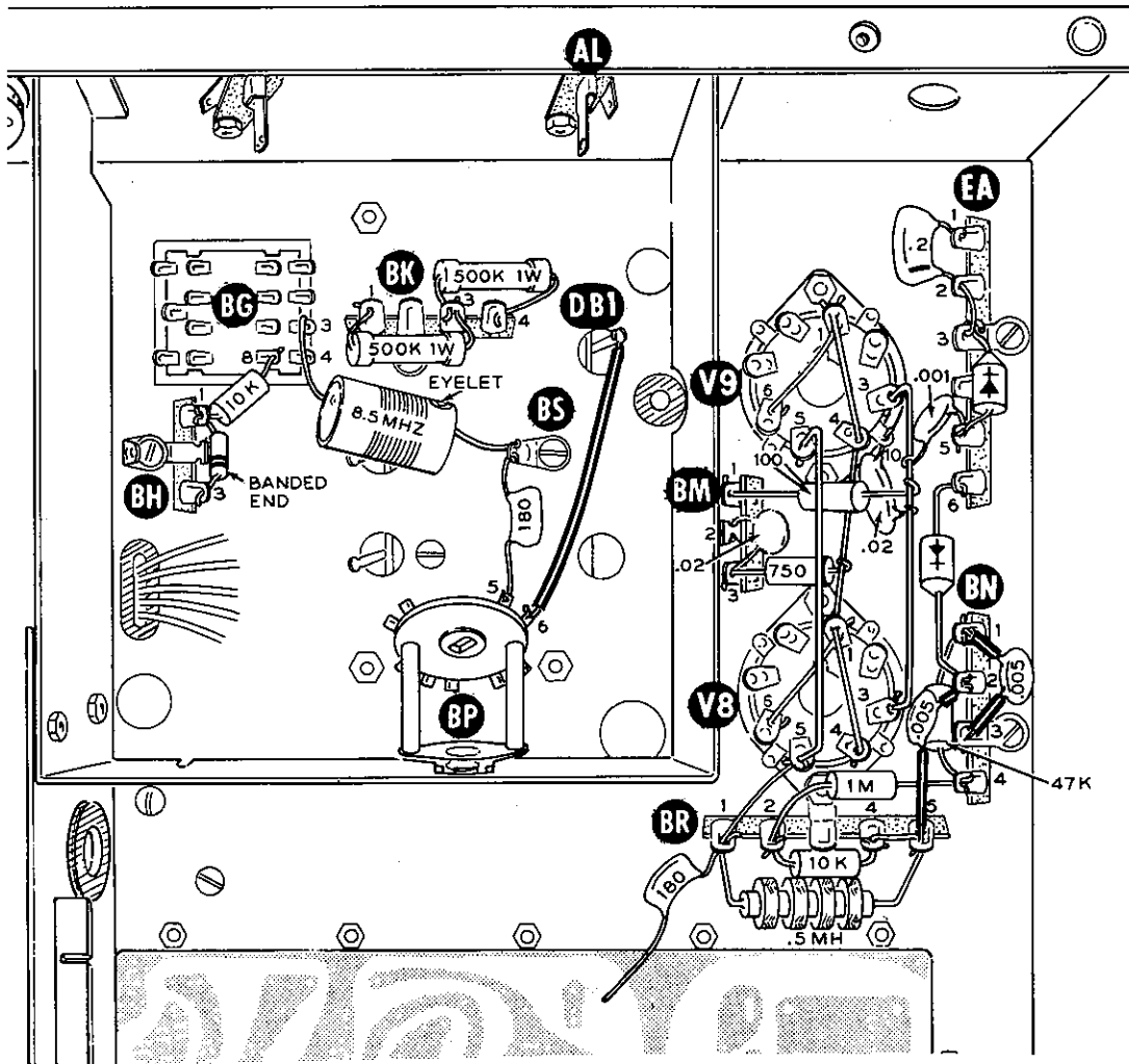
PICTORIAL 3-5
