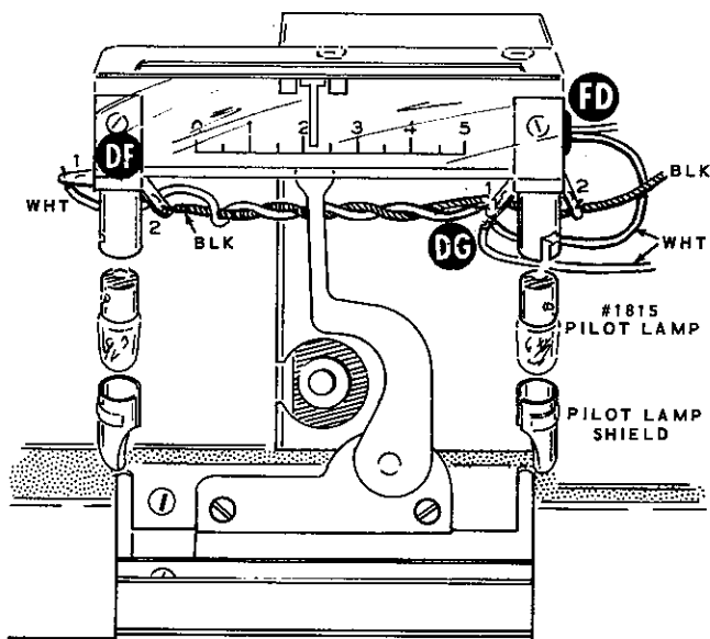
Detail 3-10A
