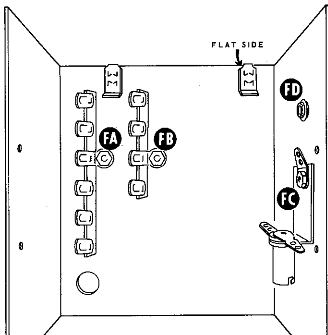
PICTORIAL 3-7
