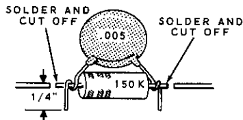
Detail 3-4A
