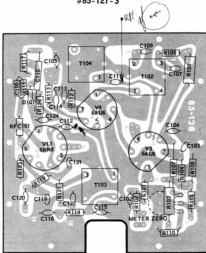
IF CIRCUIT BOARD #85-128-2
