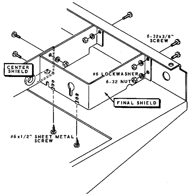
Detail 2-2T
