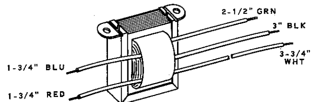
Detail 2-2H
