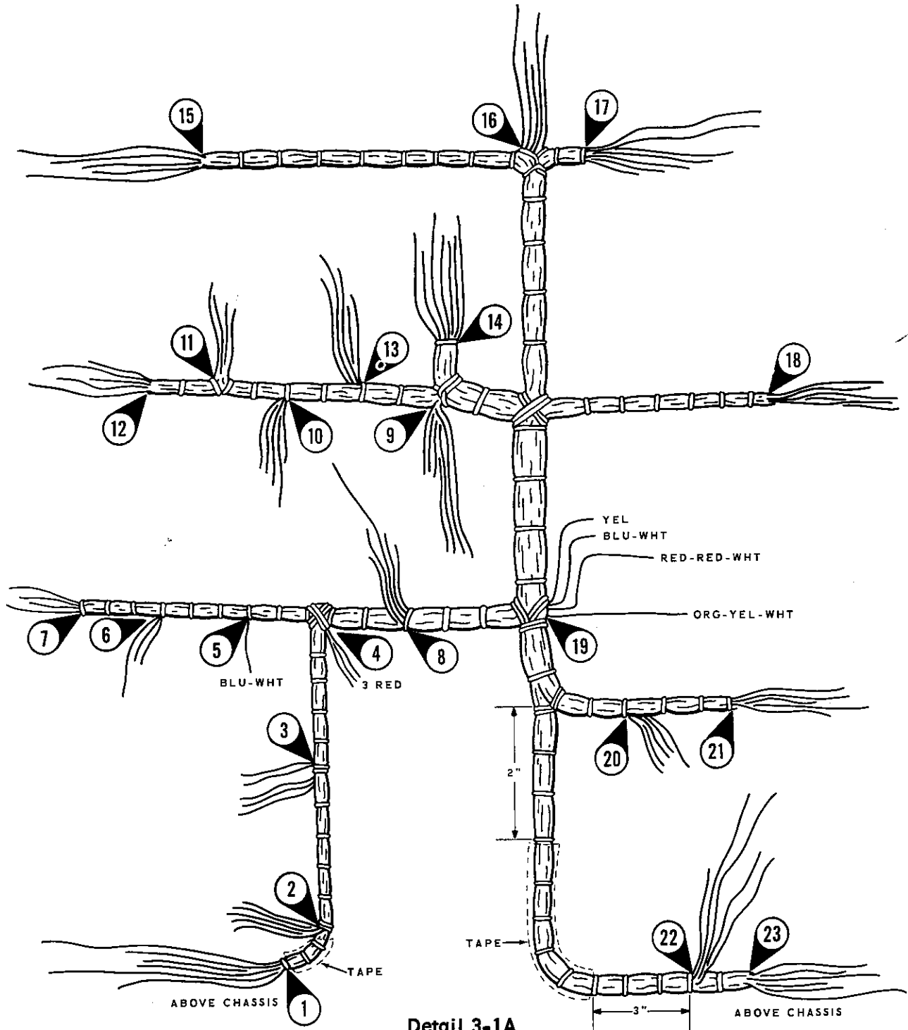
Detail 3-1A
