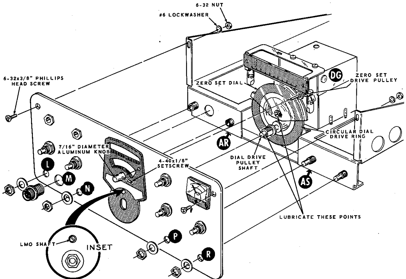
PICTORIAL 3-16
