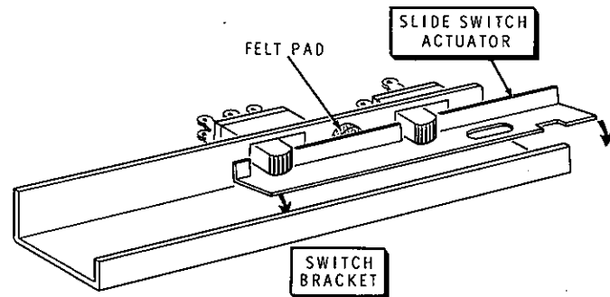
Detail 2-2C
