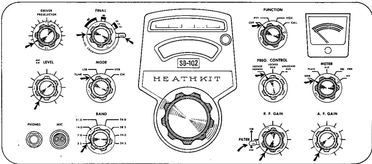
PICTORIAL 3-26
