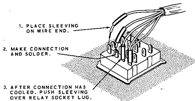
Detail 3-1B
