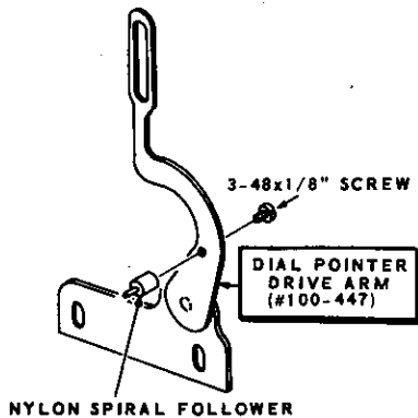
Detail 3-9A
