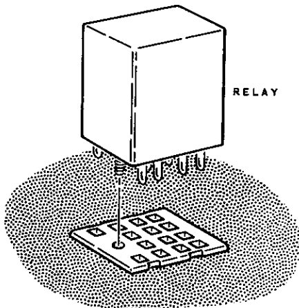
Detail 3-21B
