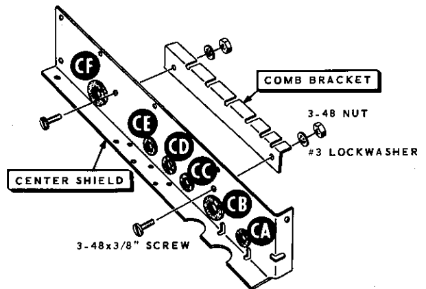
Detail 2-2F
