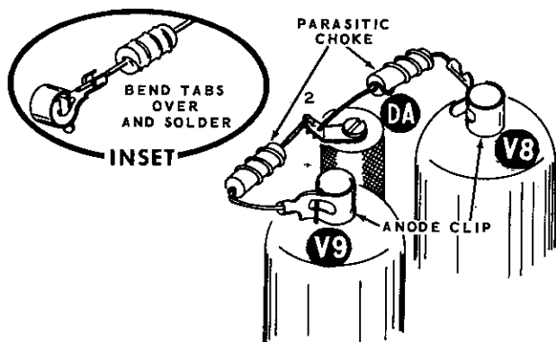
Detail 3-6B
