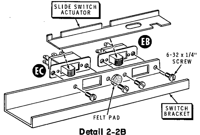
Detail 2-2B
