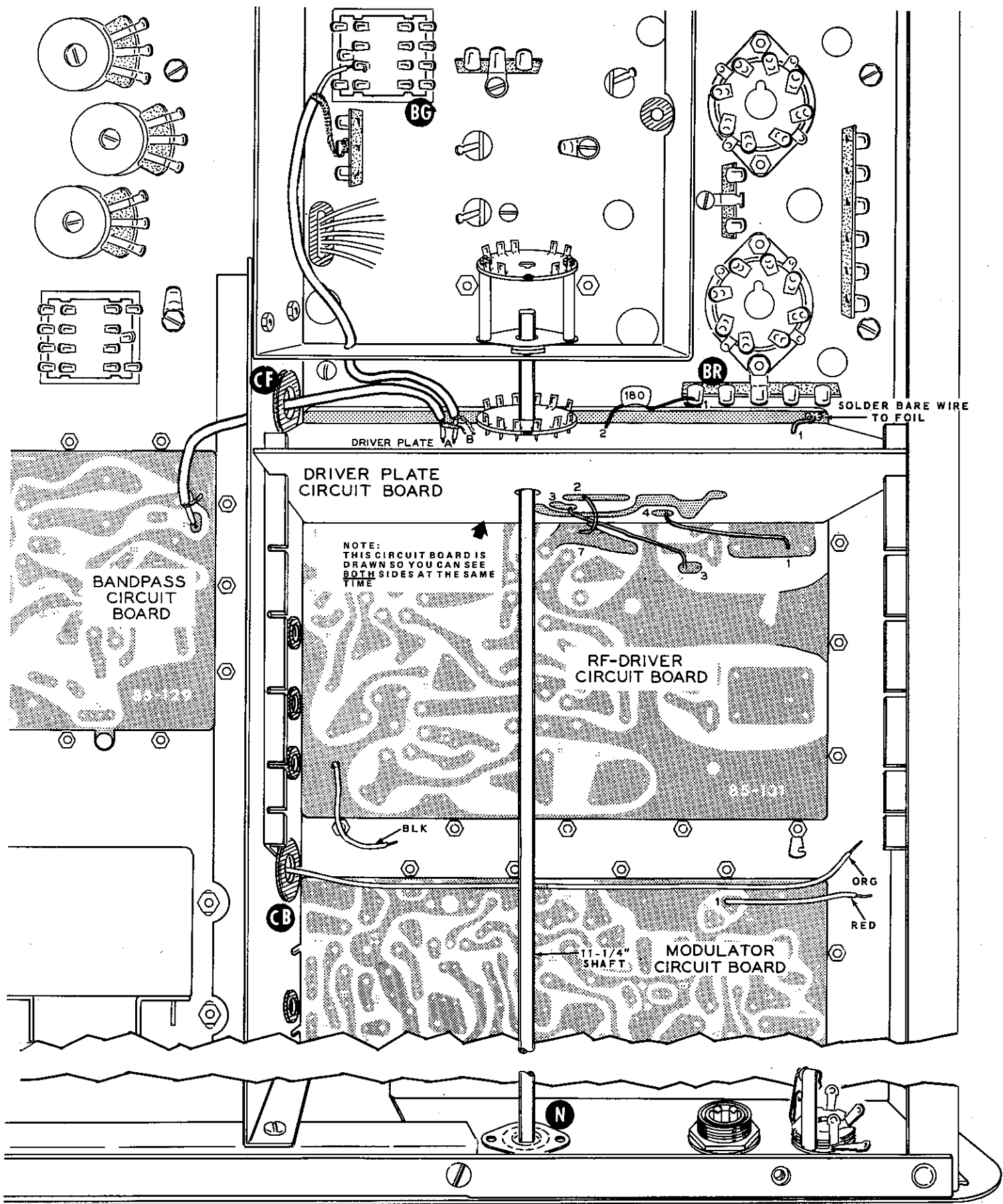
PICTORIAL 3-22
