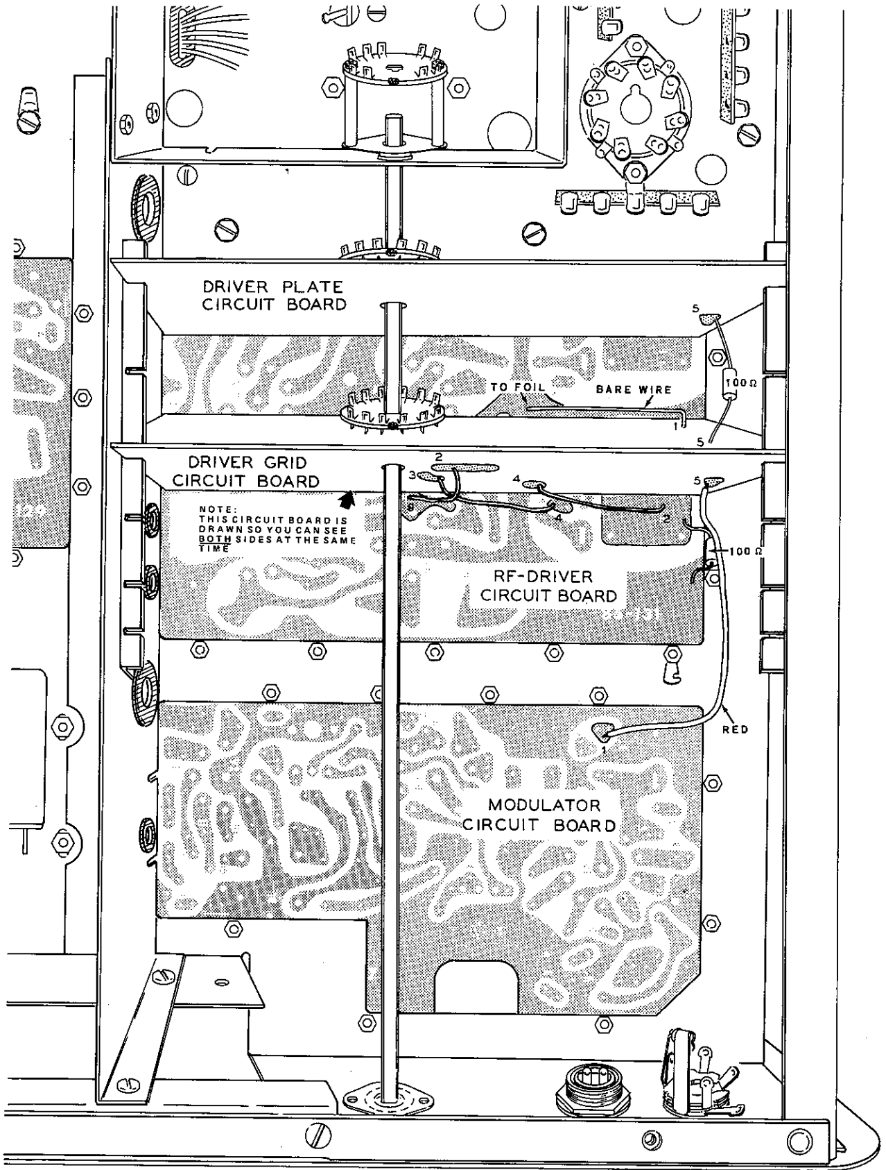
PICTORIAL 3-23
