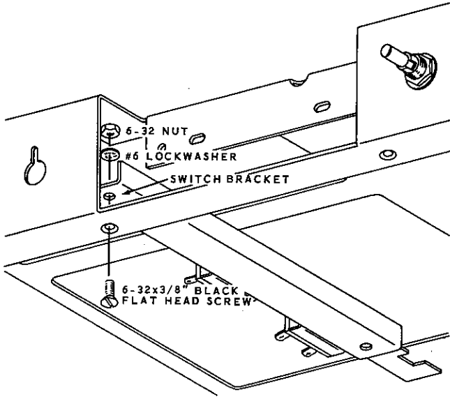
Detail 2-2D
