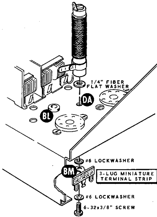
Detail 2-2R
