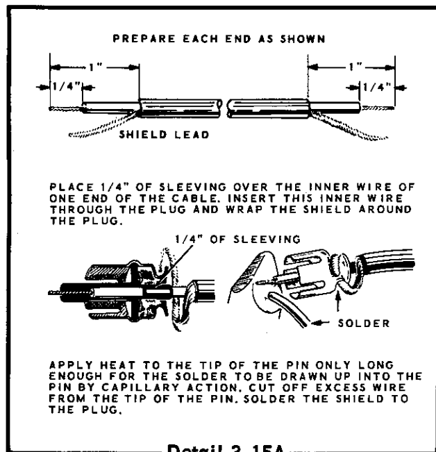
Detail 3-15A
