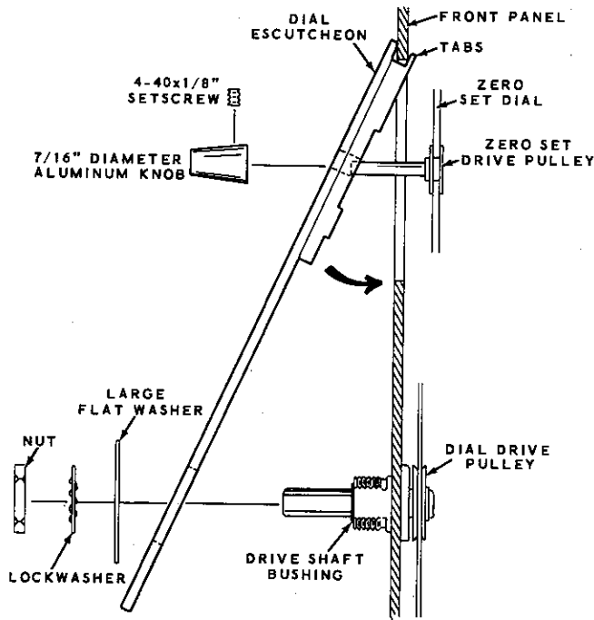
Detail 3-16A
