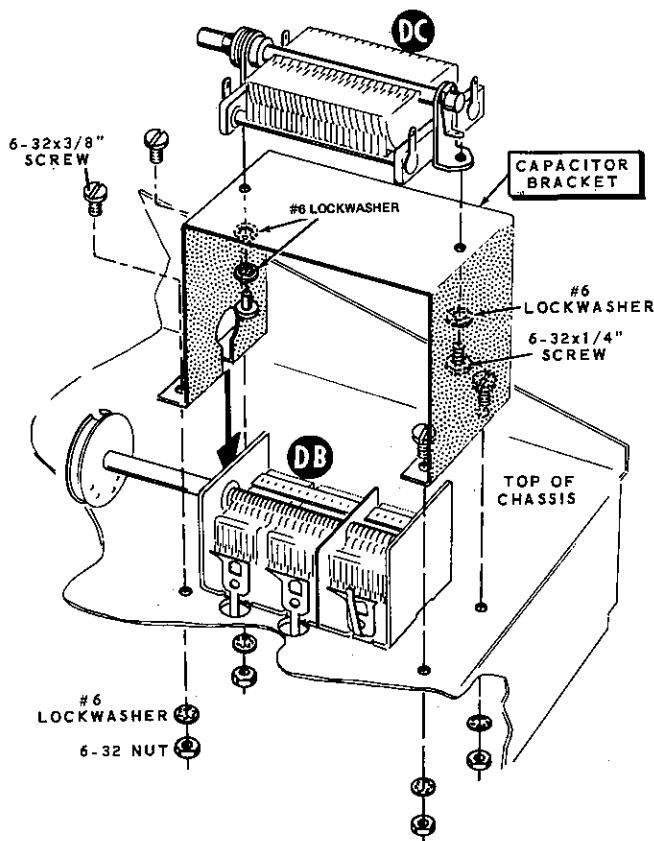
Detail 2-2Q
