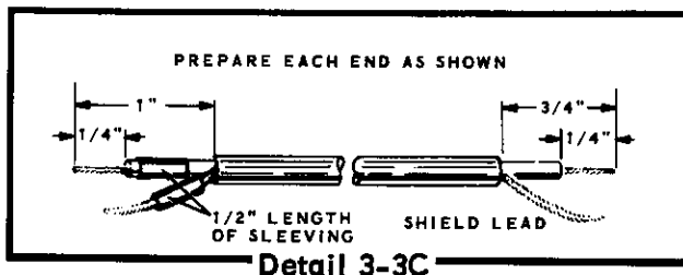
Detail 3-3C
