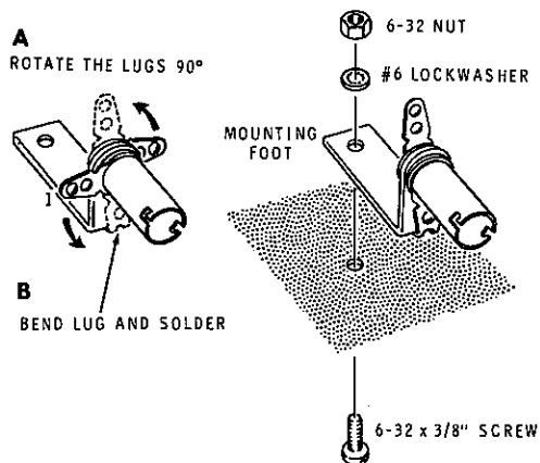
Detail 3-17A
