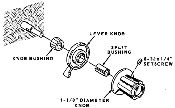
Detail 3-26A
