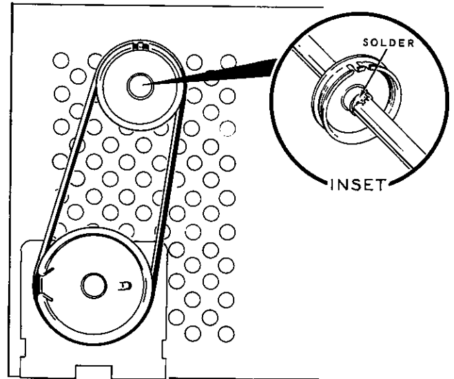
PICTORIAL 3-20
