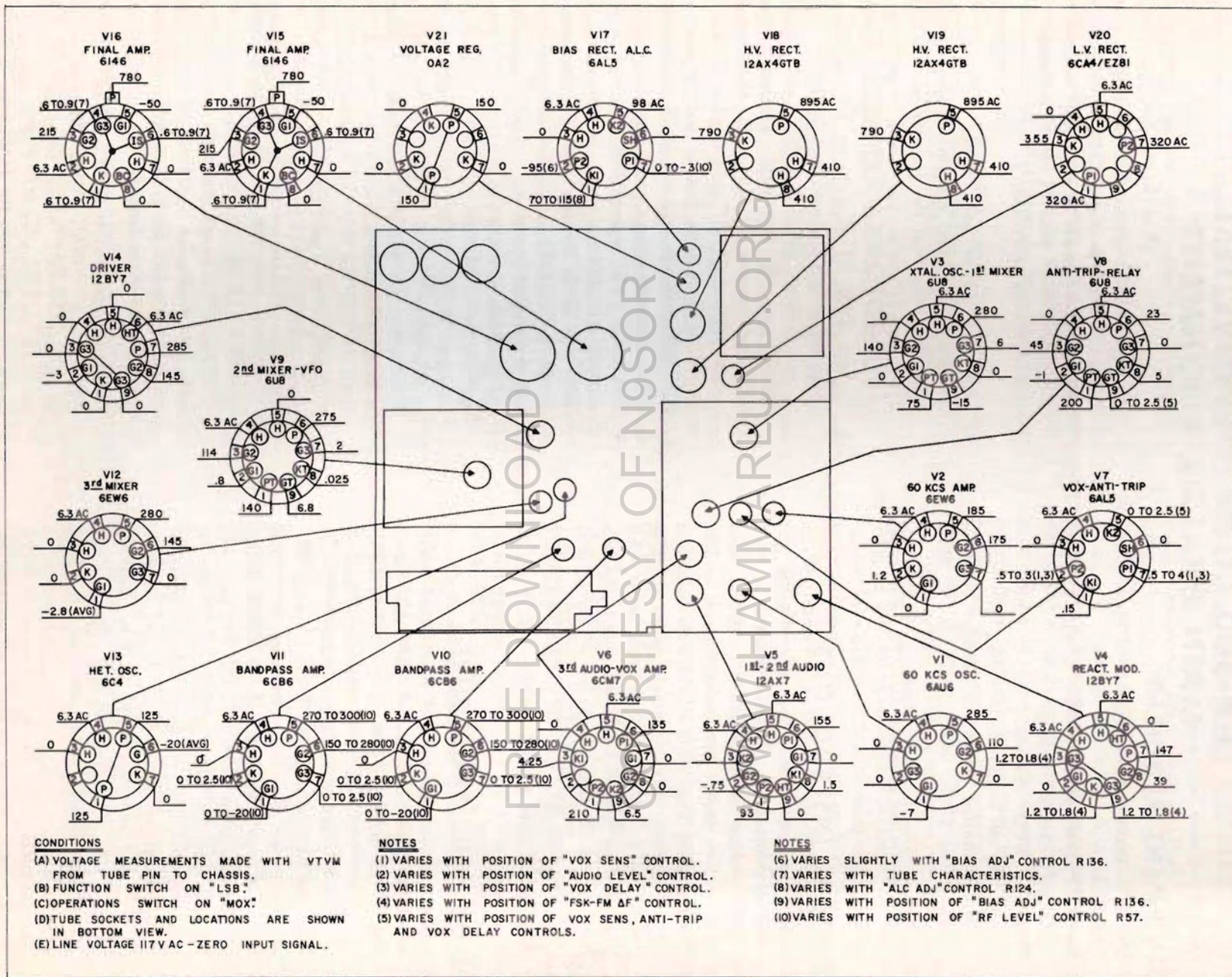
Figure 11. Voltage Chart
