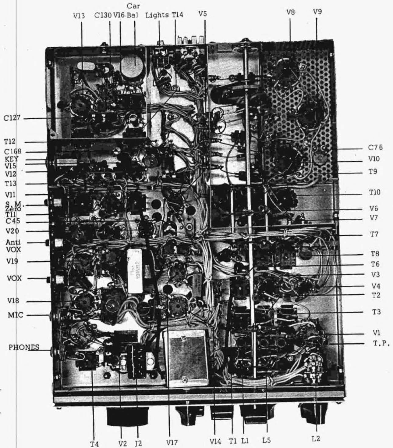
Figure 11 BOTTOM VIEW
