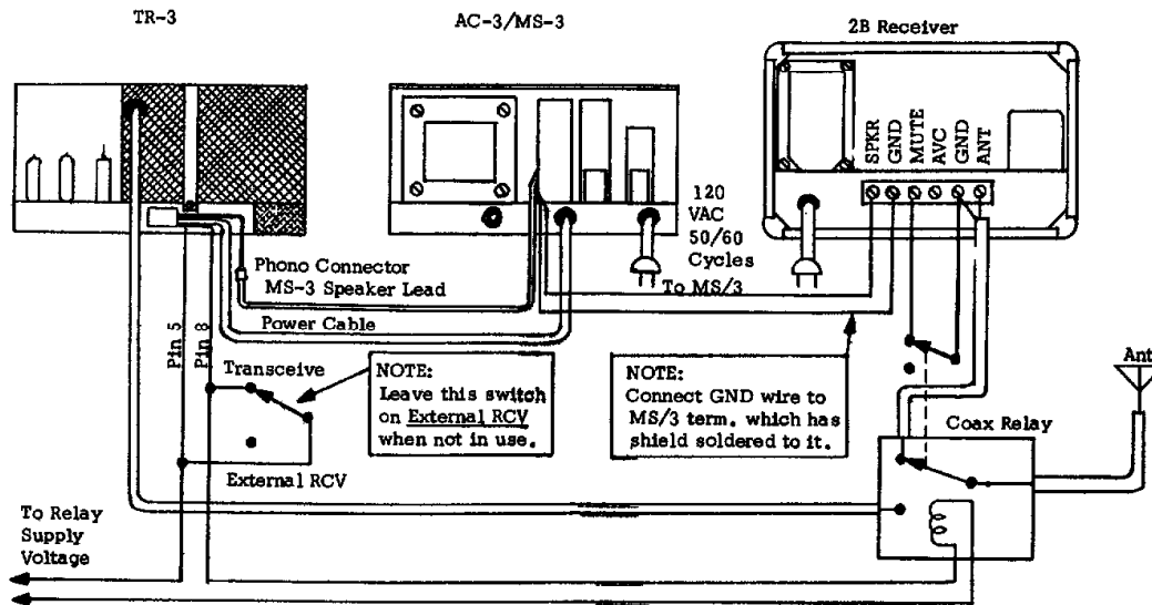
FIG. 3 USING THE TR-3 WITH AN EXTERNAL RECEIVER
