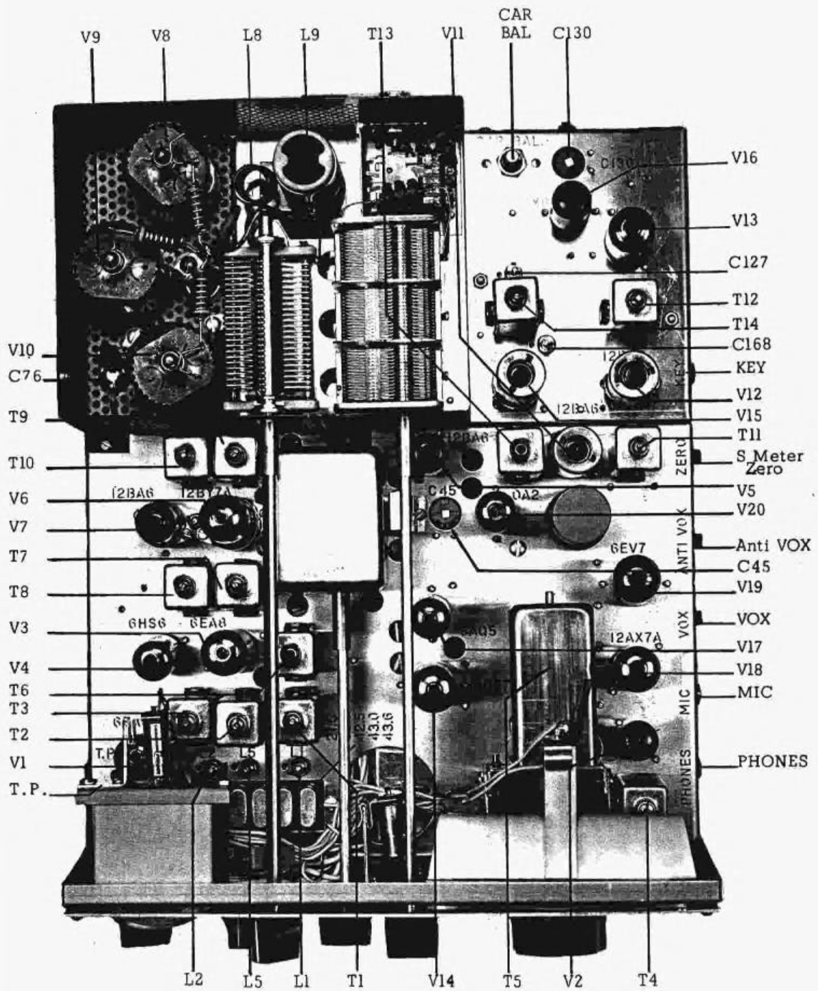
Figure 10 TOP VIEW
