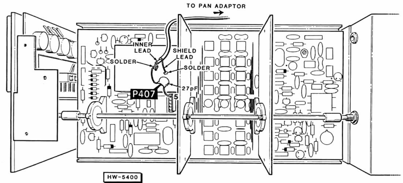
PICTORIAL 3-3
