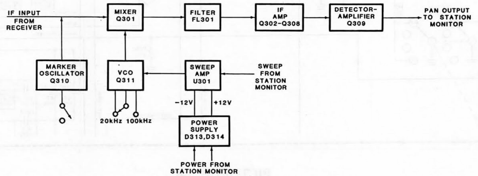
BLOCK DIAGRAM
