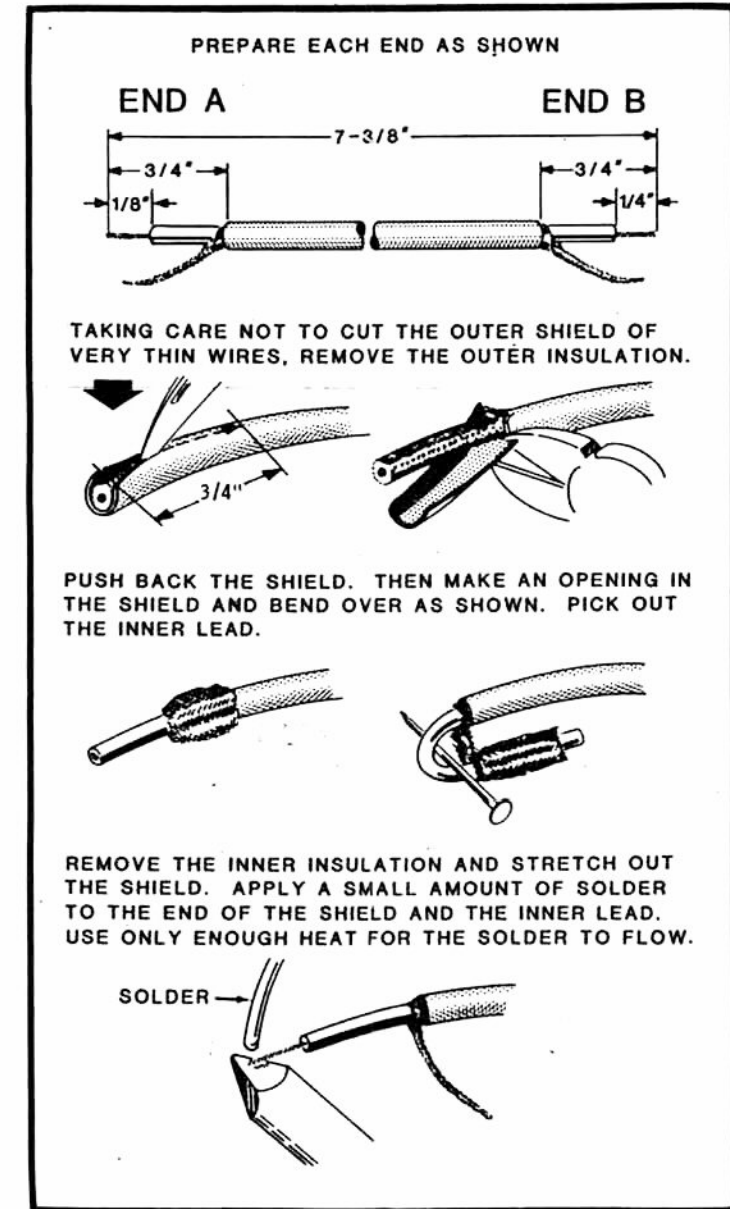
Detail 1-8D
