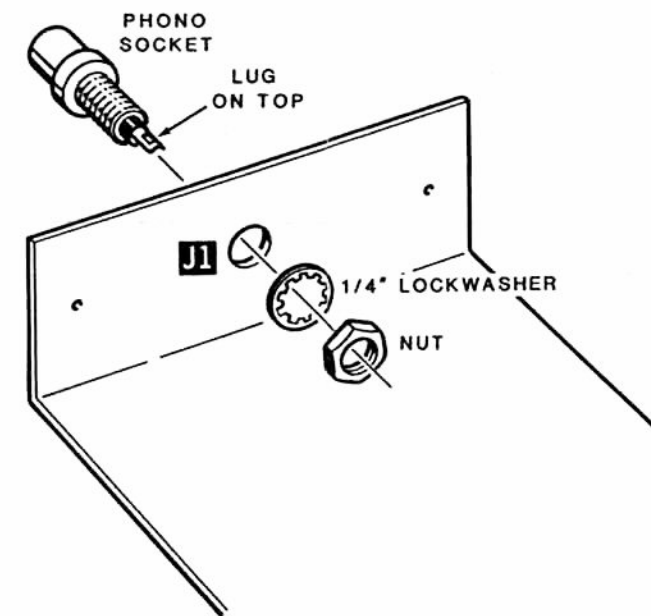
Detail 1-7A
