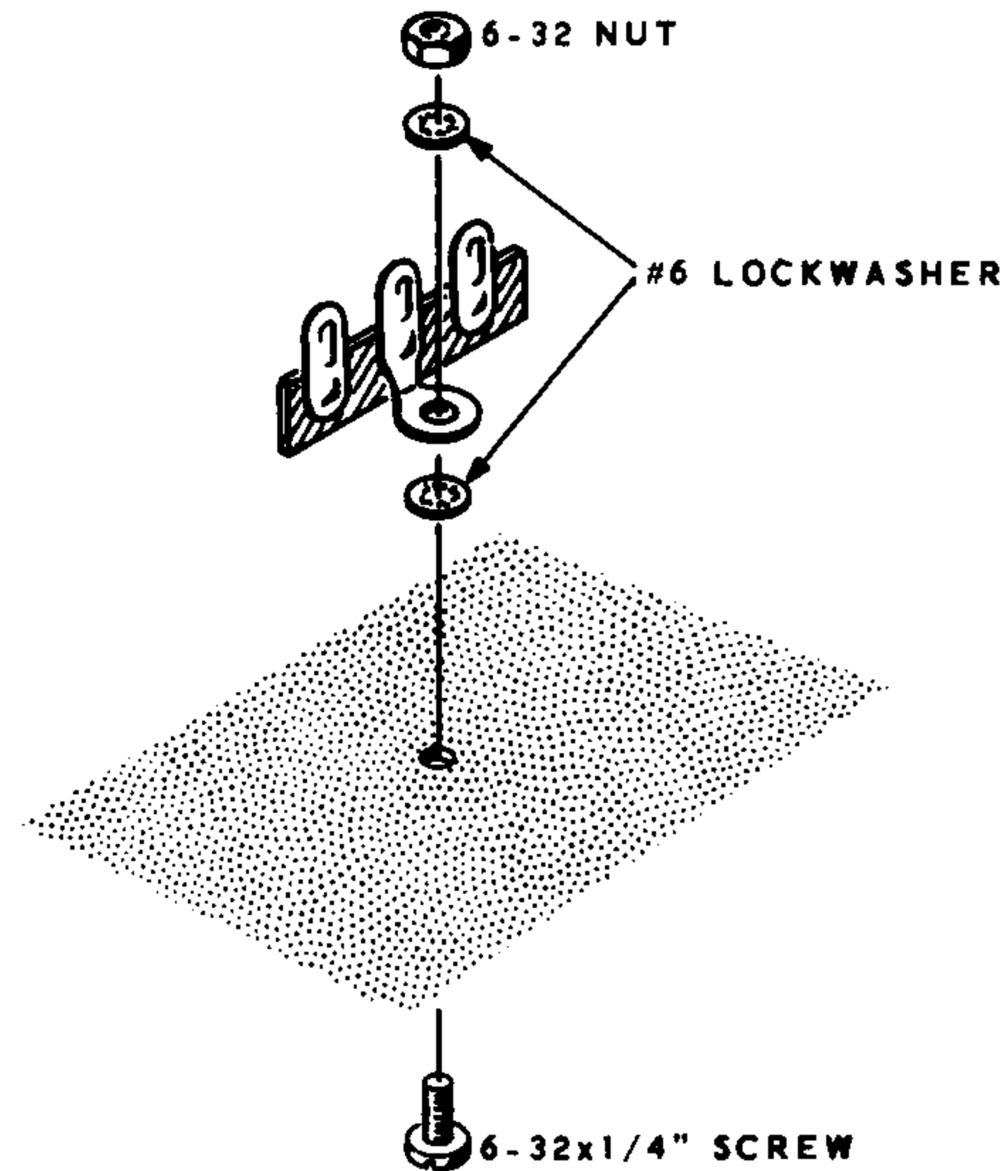
Detail 1B
