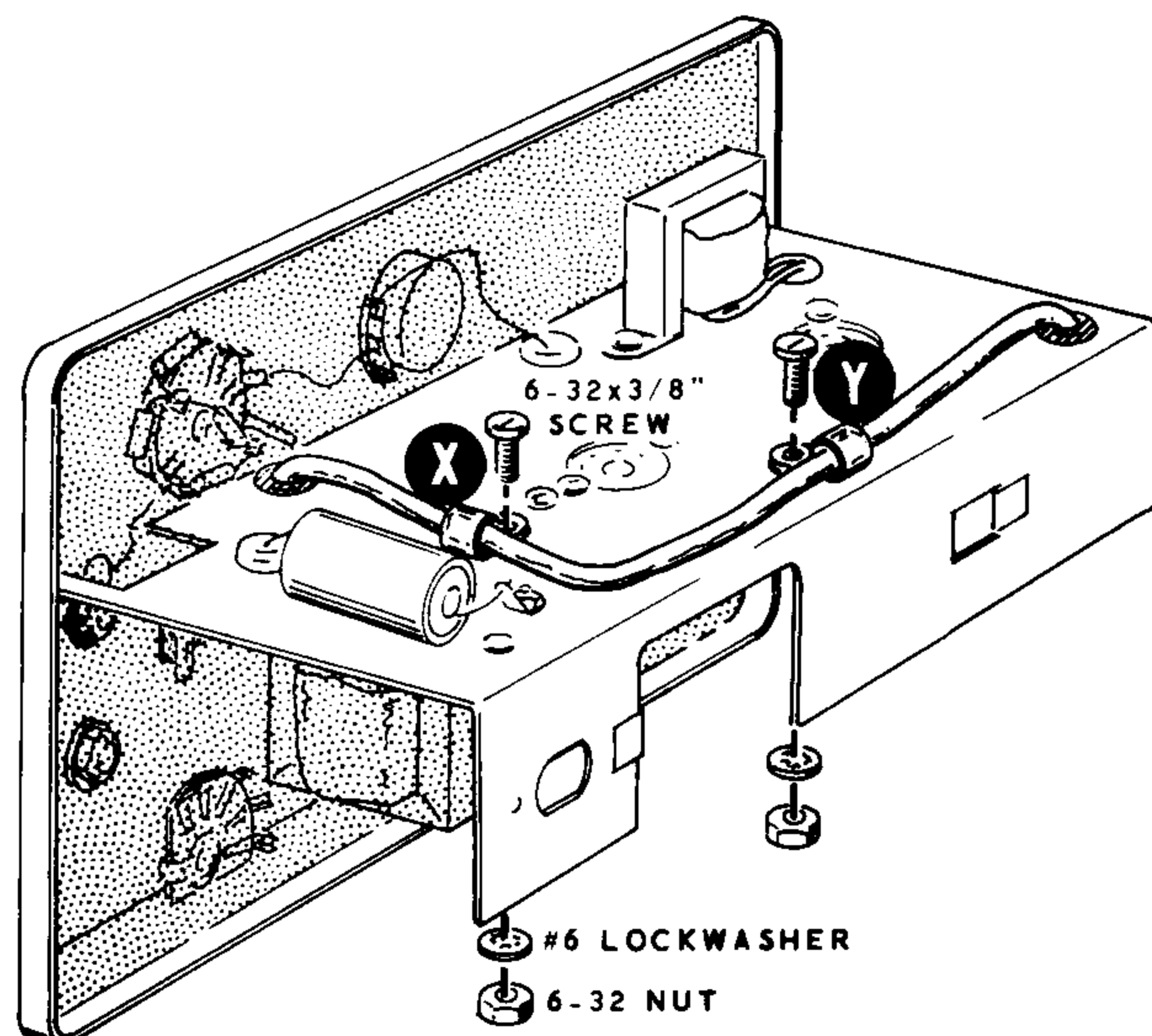
Detail 3C
