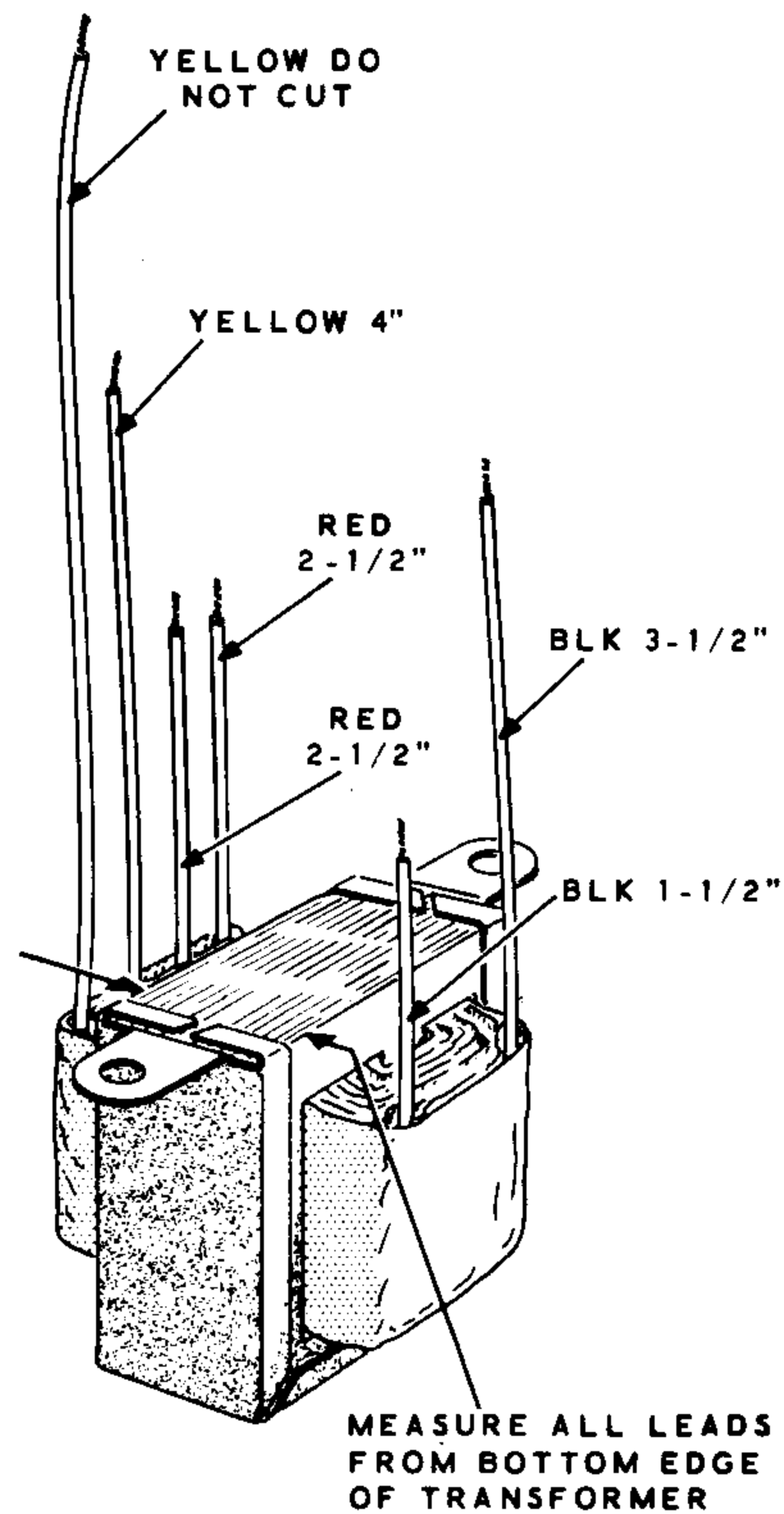
Detail 1J
