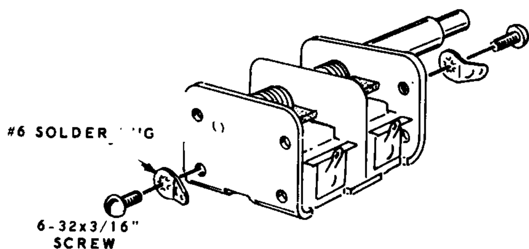
Detail 5A
