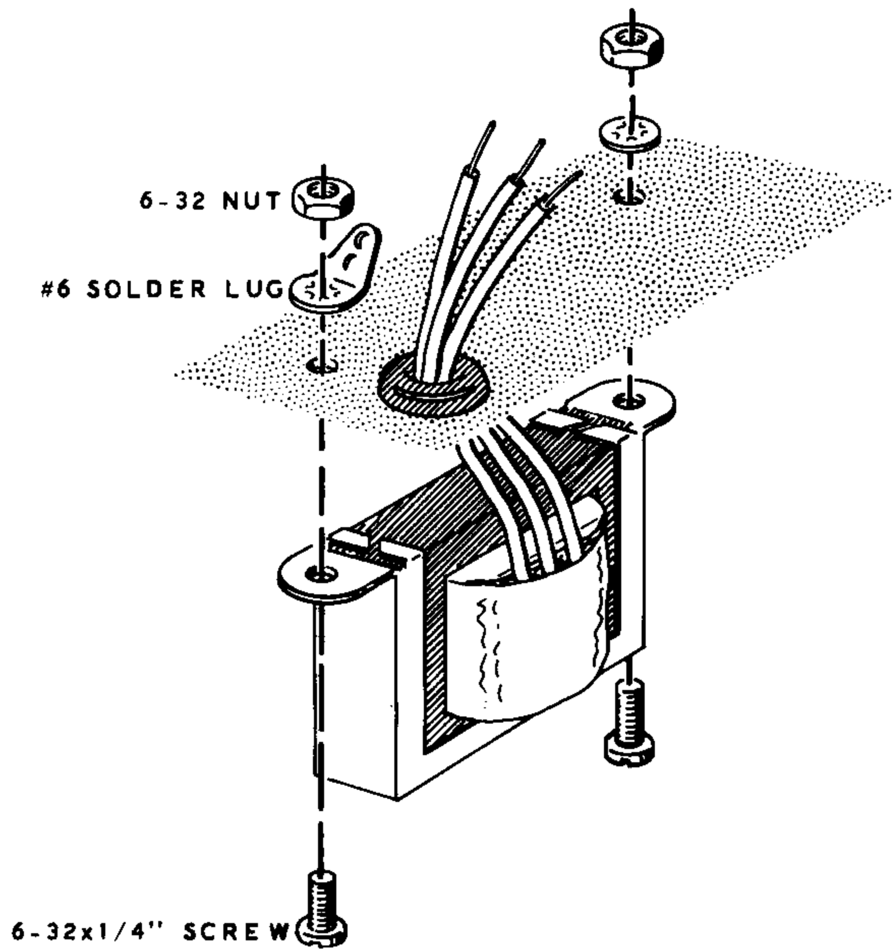
Detail 1C
