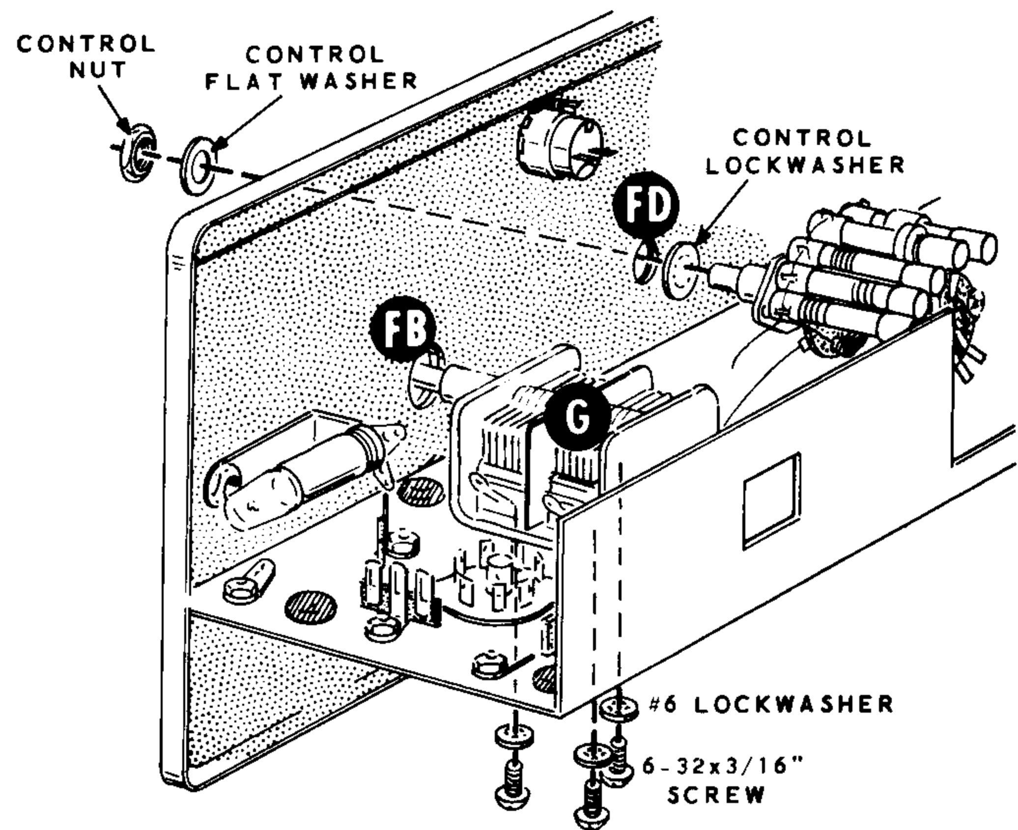
Detail 5B
