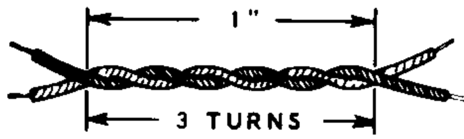
Detail 3A
