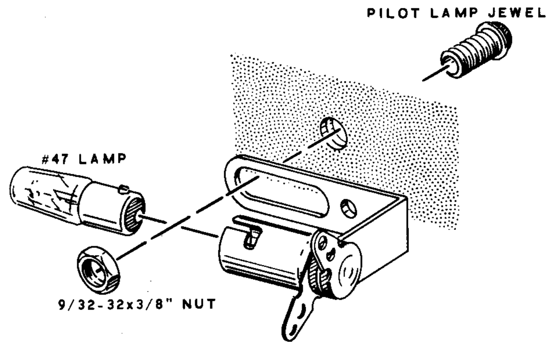
Detail 1H
