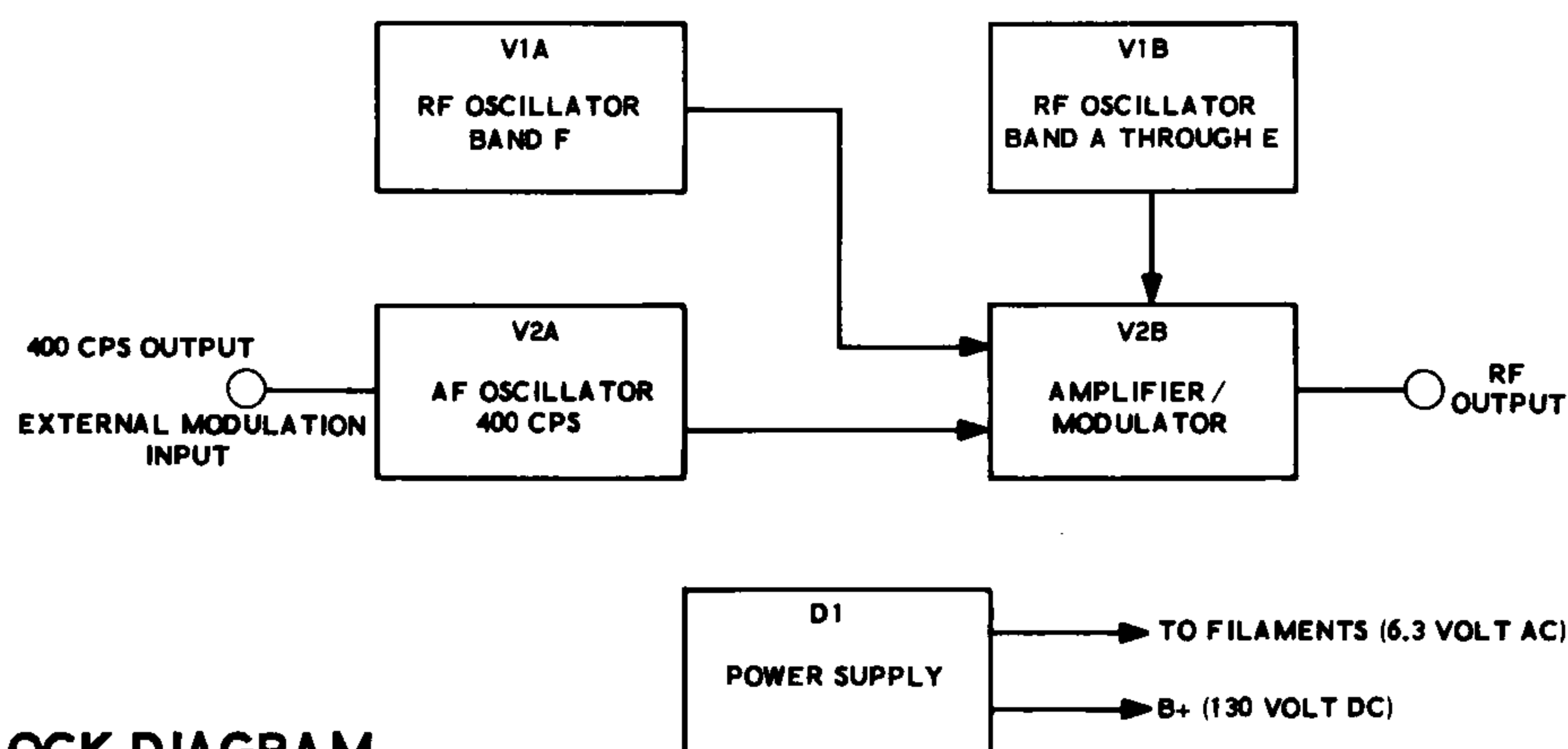
BLOCK DIAGRAM
