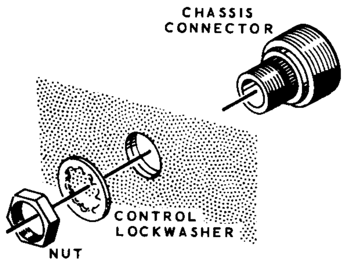
Detail 1G
