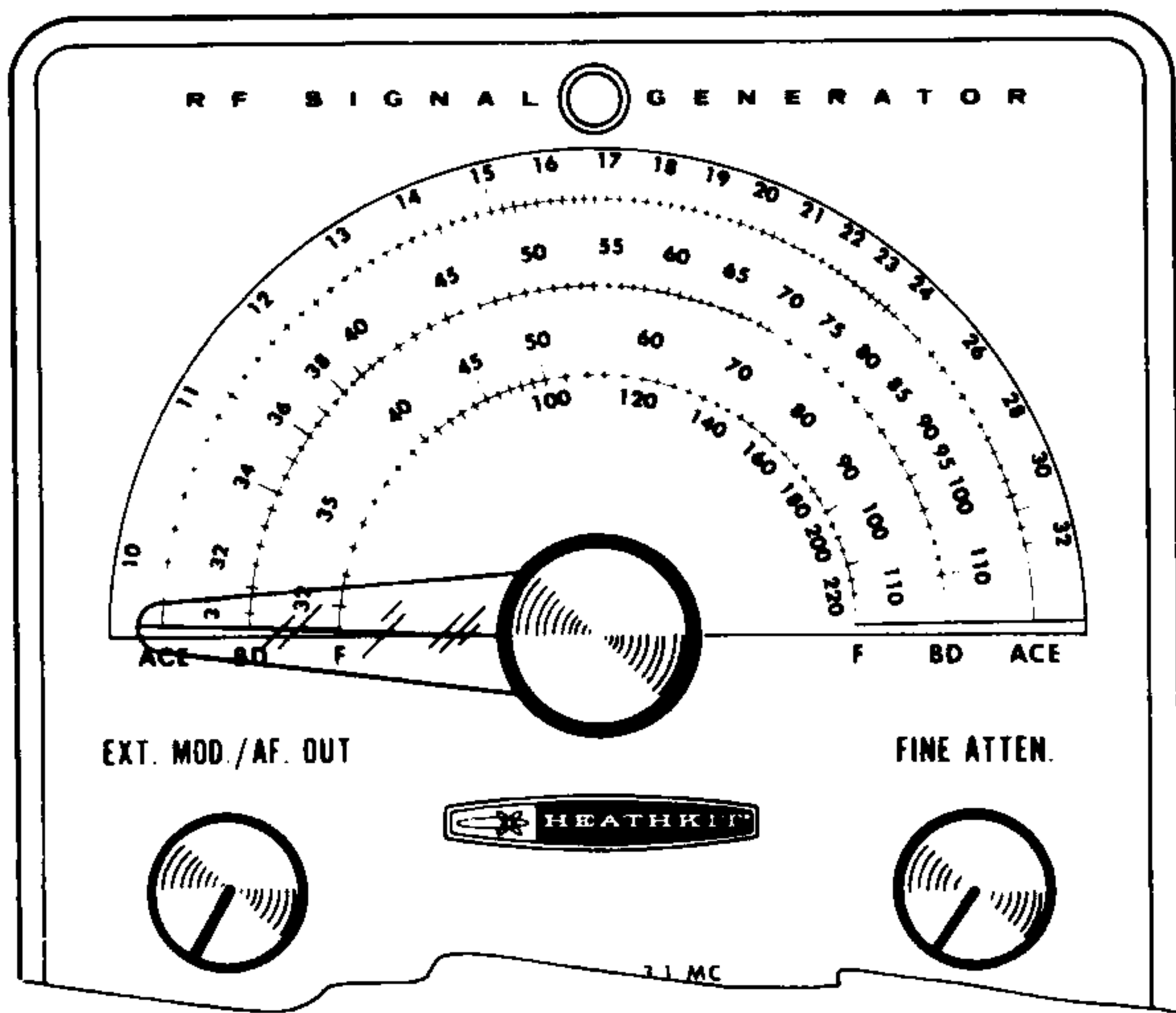
Detail 6A
