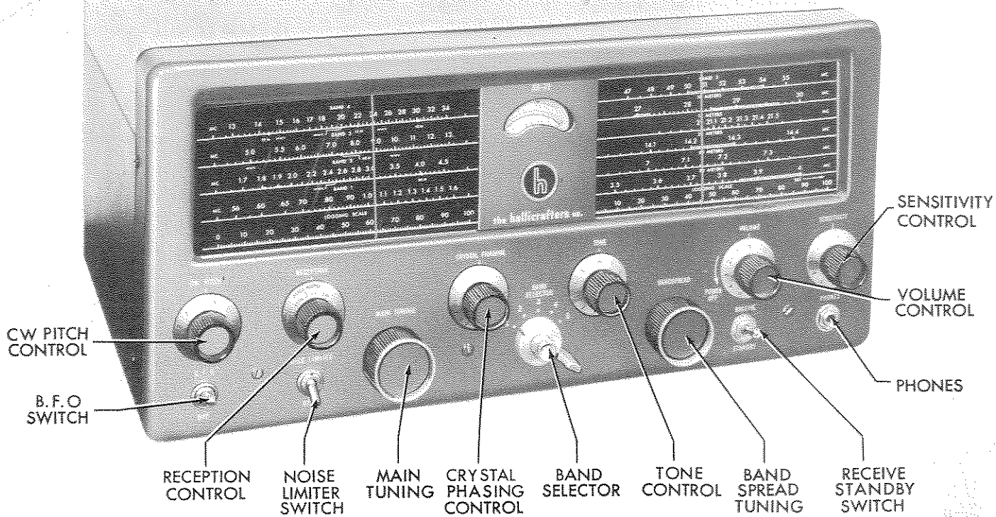
FIG. 1. COMMUNICATIONS RECEIVER MODEL SX-71
