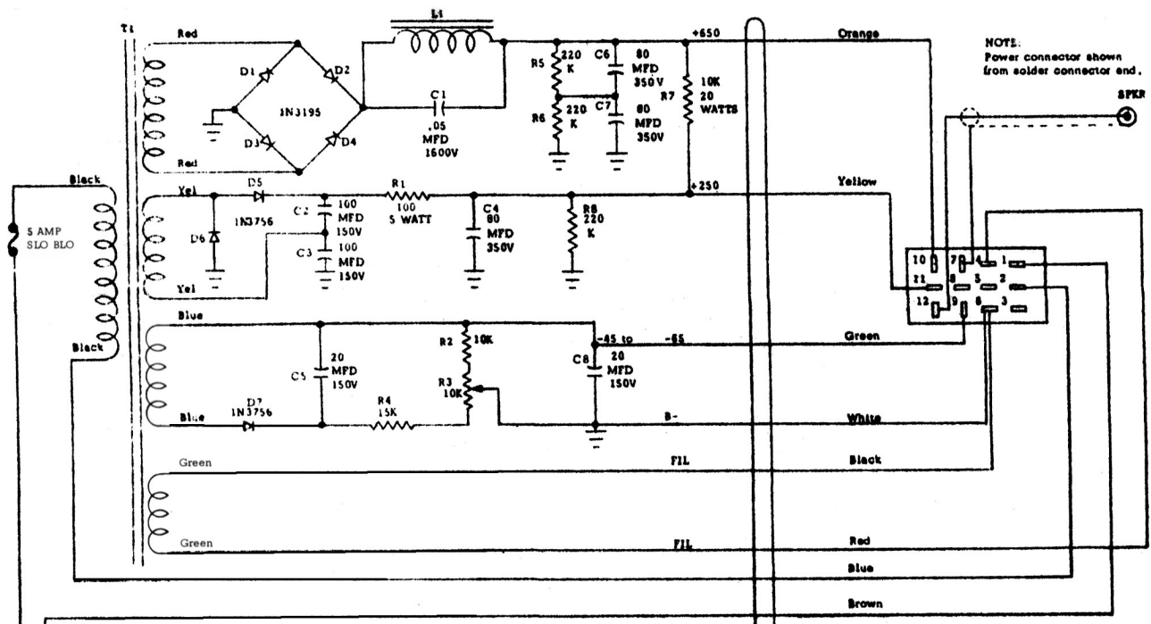
SCHEMATIC DIAGRAM MODEL AC-3 POWER SUPPLY
