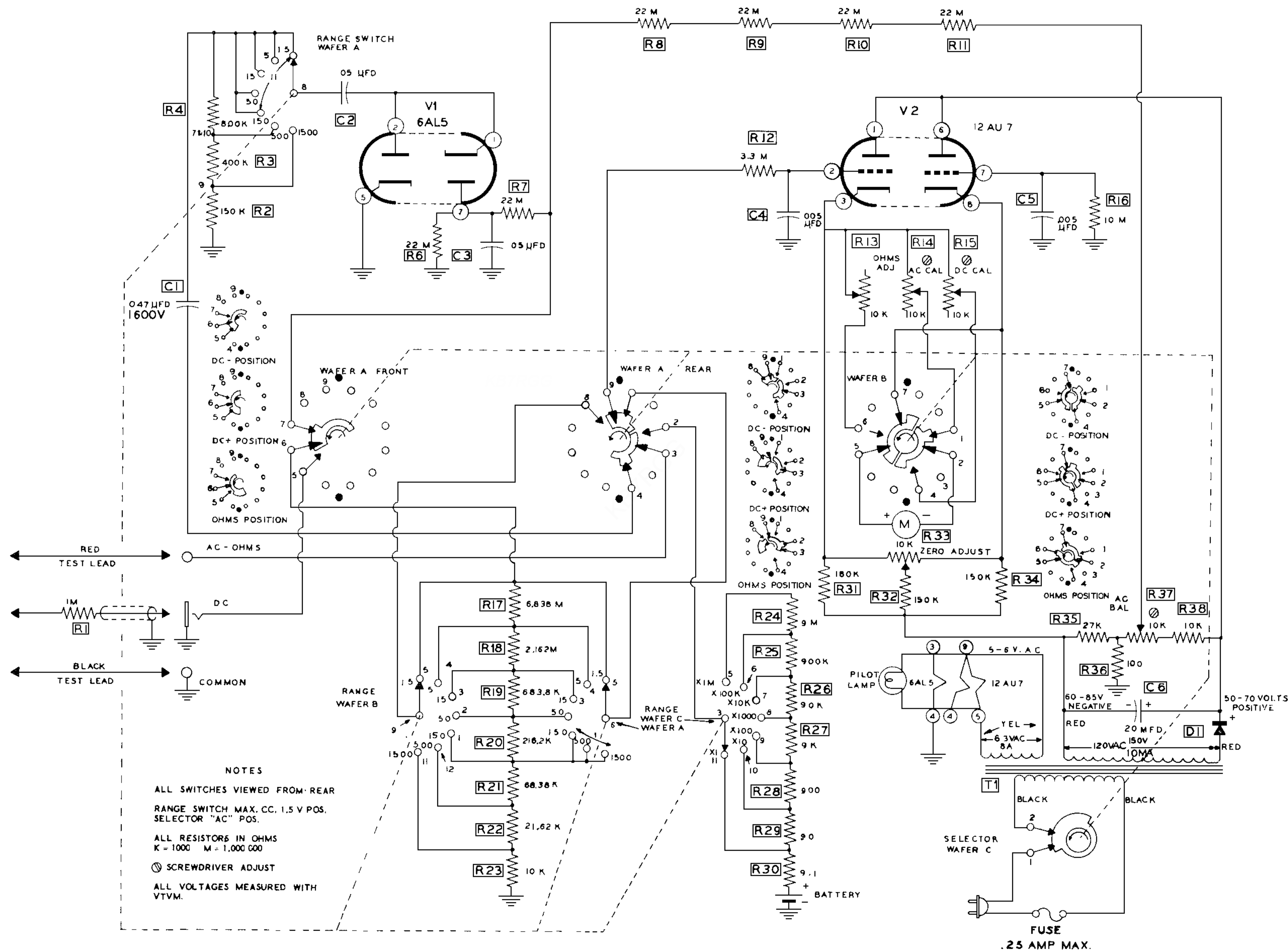
Model IM-32 VTVM.
